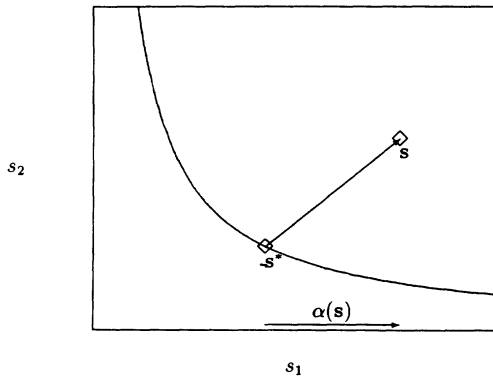
FIG. 3. The geometric solution; the hypersurface \mathbf{s}^* satisfies \prod_j s_j^* = 2^d .
